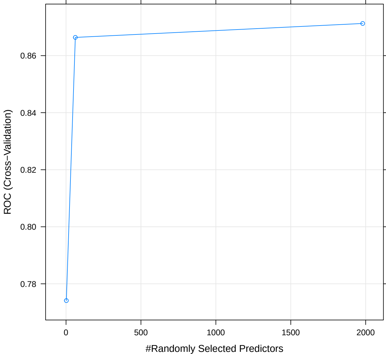
C: Microbiome Species Abundance Data,1981 Microbiome species;187 Patients Model:Random forest model by applying cross validation 5 folds
